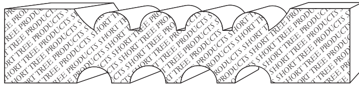
BLC 135 3/4" x 3 1/2"
